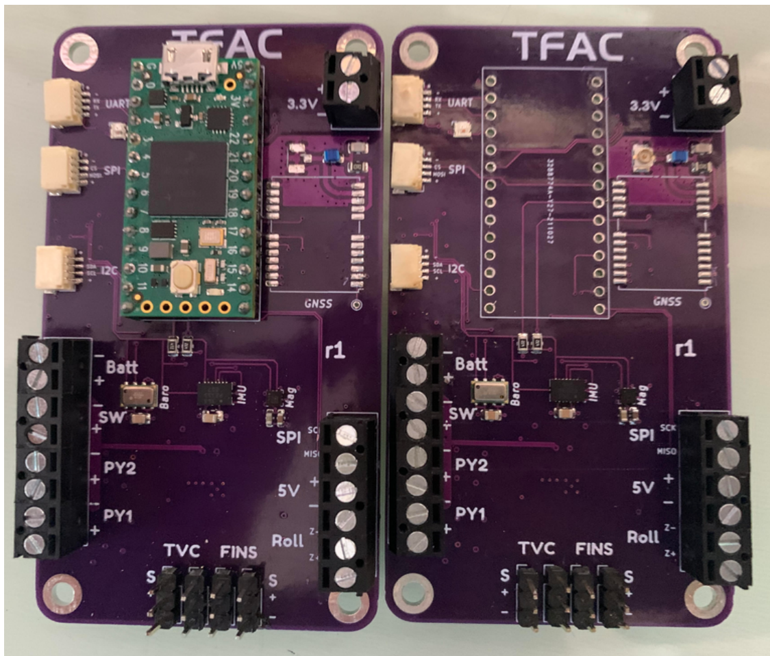
The two TFAC flight computers
