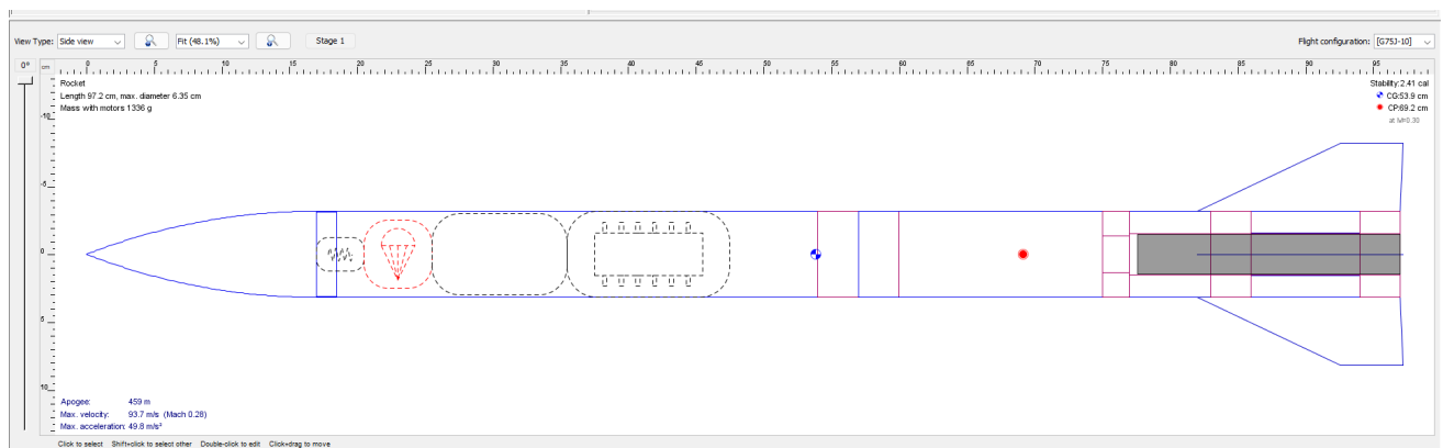
AltusAer OpenRocket model
